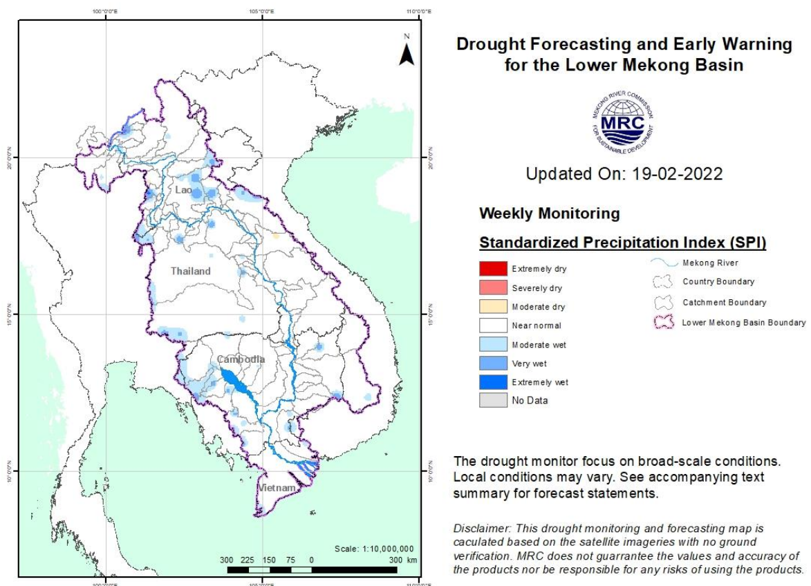
Figure 14: Weekly standardised precipitation index from Feb 13 to 19.
